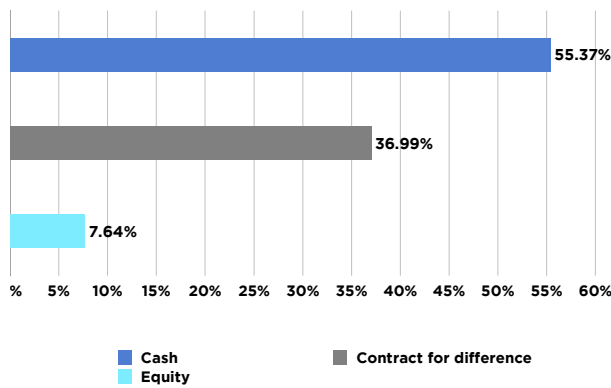
Exposure Statistics
